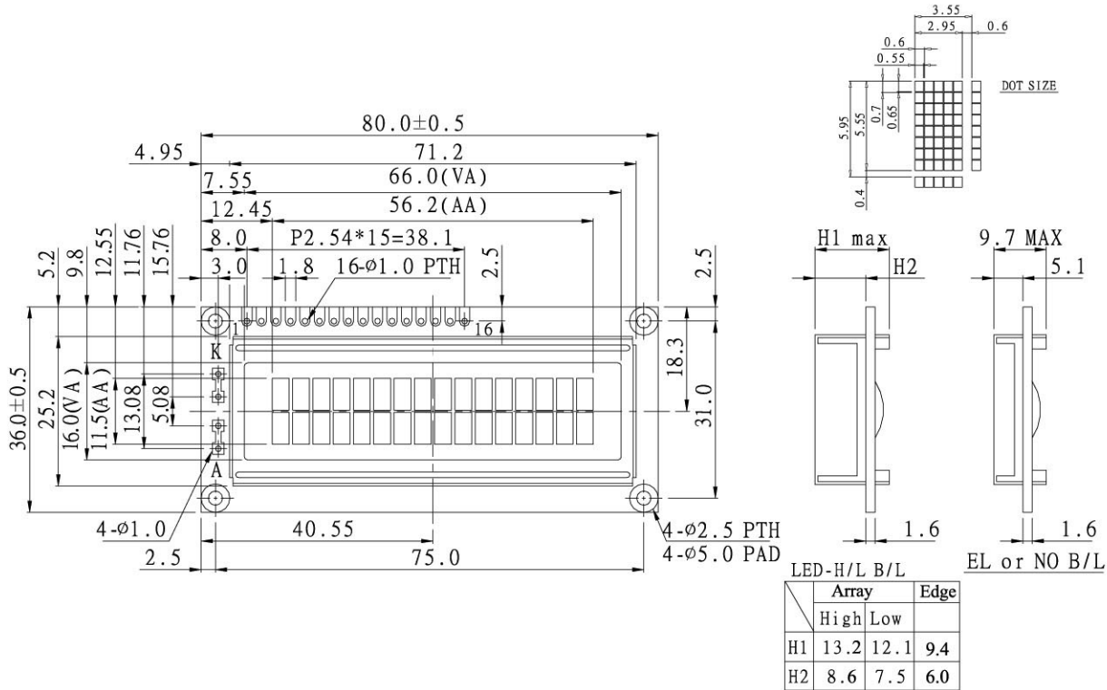
Dimension drawing
