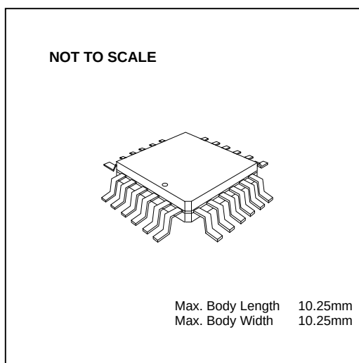
FX315LG 24-pin quad plastic encapsulated bent and cropped (L1)
