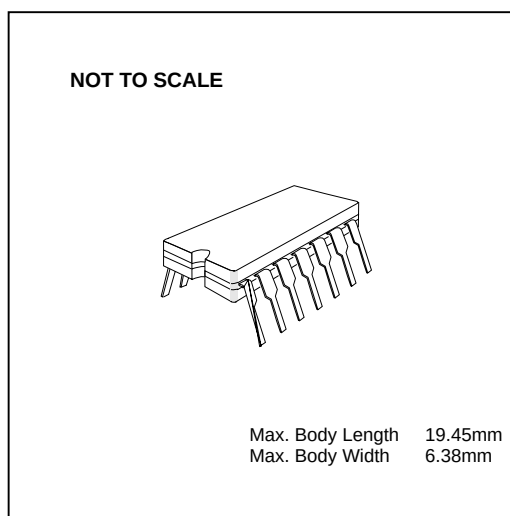
FX315J 14-pin cerdip DIL (J1)
