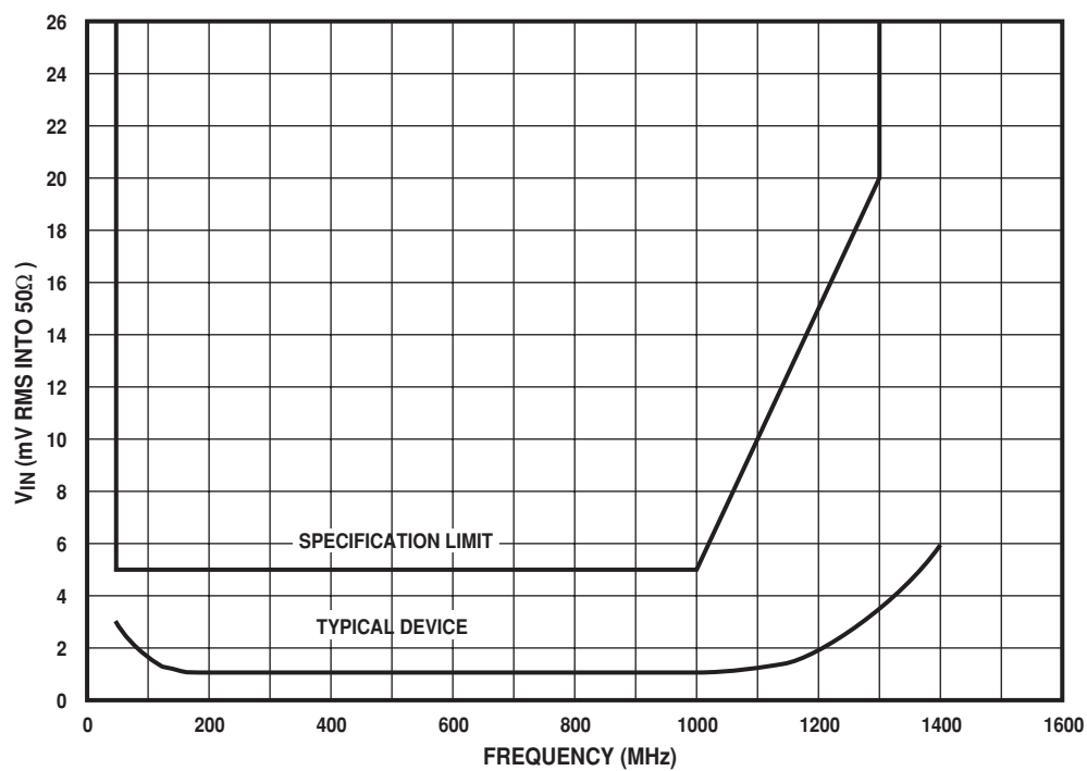
Fig. 5 Typical input sensitivity
